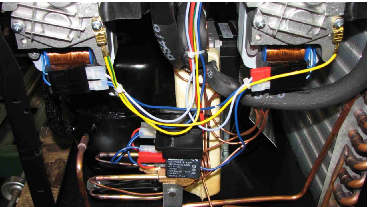
GEAR MOTORS WIRING
